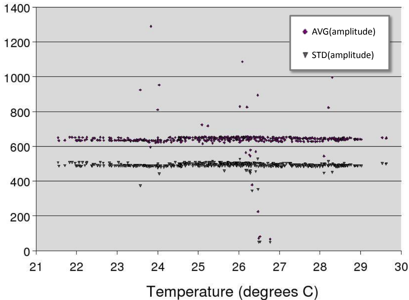
AVG(amplitude) and STD(amplitude) vs. Temperature (6 days, from 3/7/09 20:00)
