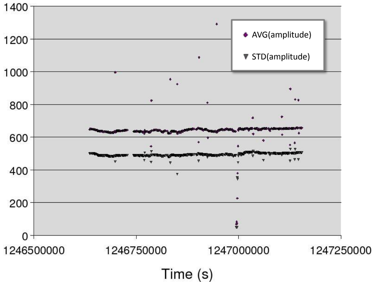
AVG(amplitude) and STD(amplitude) vs. Time (6 days, from 3/7/09 20:00)
